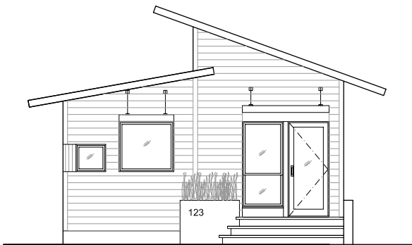
WEST ELEVATION
