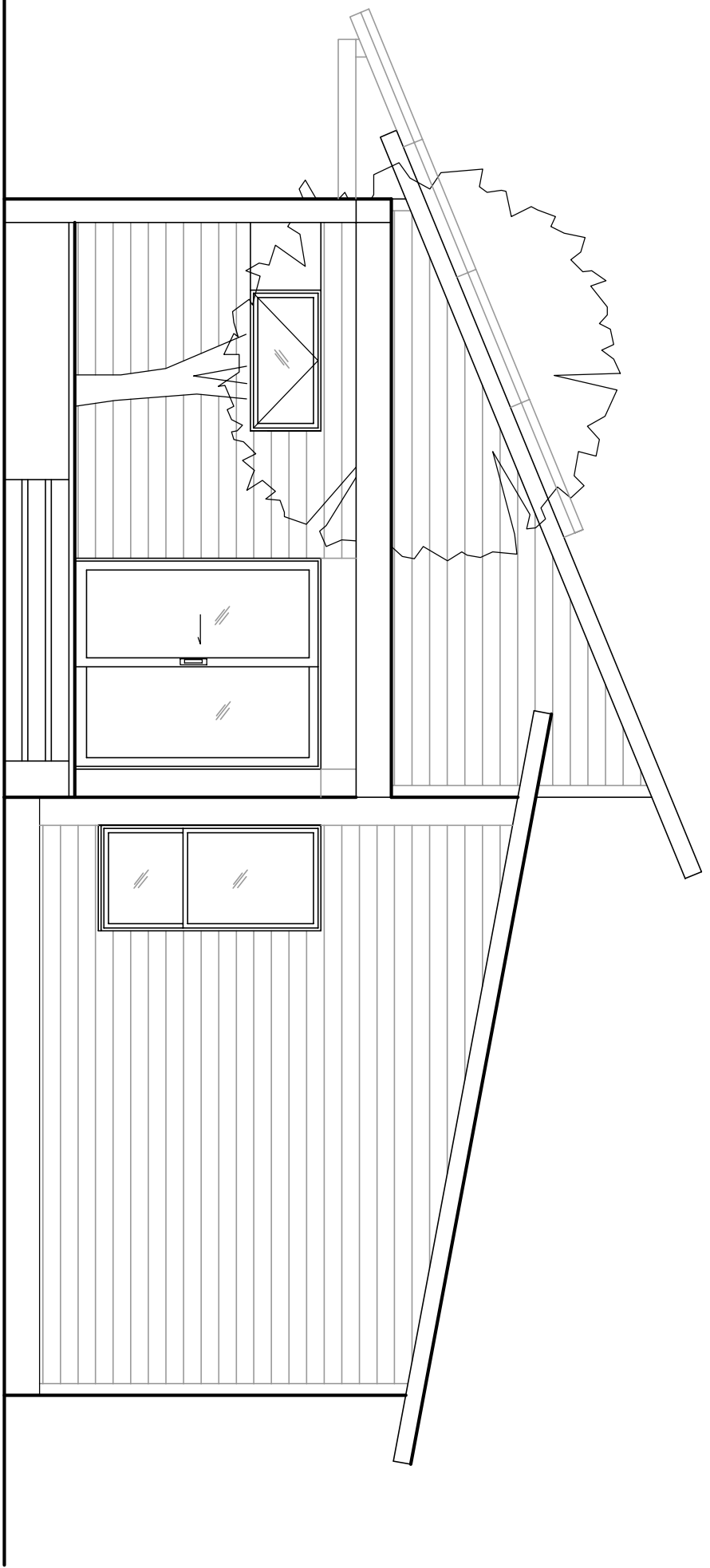
EAST ELEVATION (v.2)
